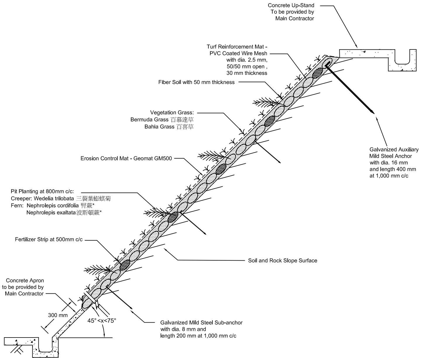
Existing Soil and Rock Slope
